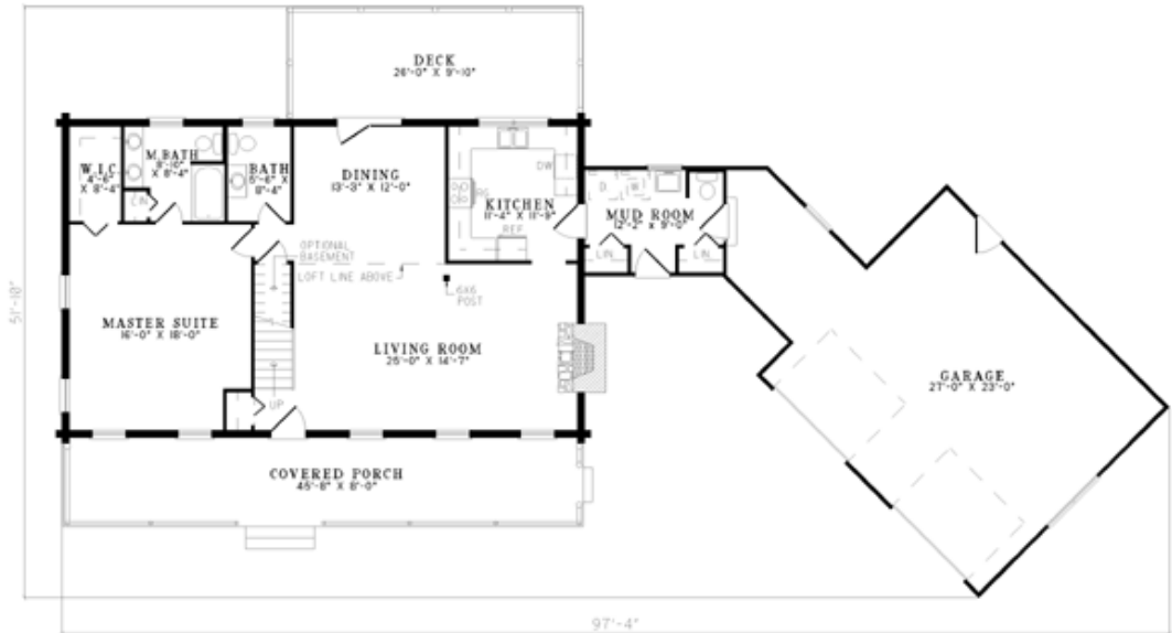
1st Floor
