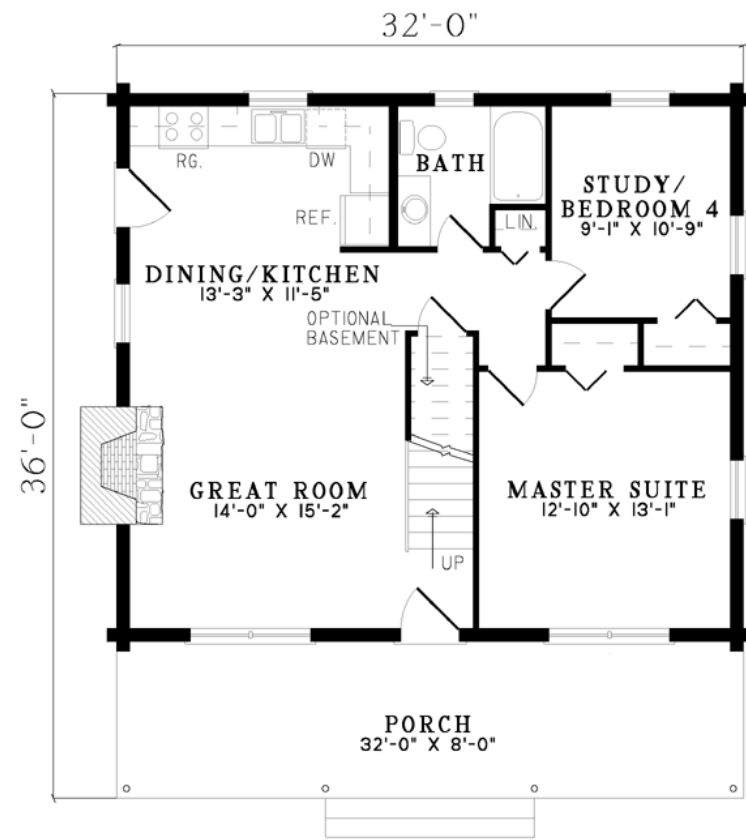
1st Floor
